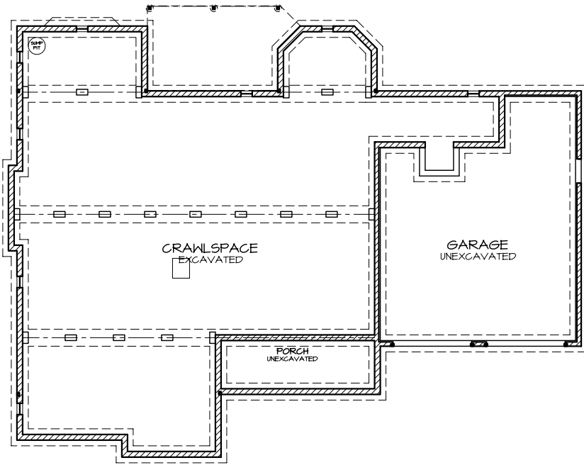
1 FOUNDATION PLAN A-3
